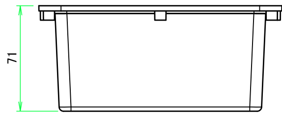
F-F (1:2.5)
